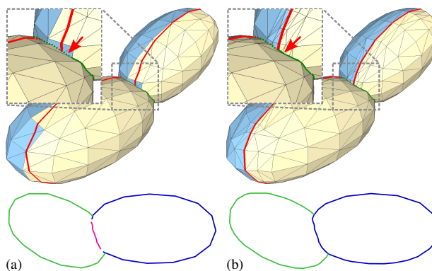
Fig. 27. Visibility of Surface Intersections. Defining visibility for curves near interpolated contours is difficult, such as the Surface Intersection curves (green). (a) Heuristics can be used to get reasonable interpolated contour visibility in simple cases, but the Surface Intersection curves still give errors (red arrow). (b) Our method allows to compute accurate visibility for all curves, preventing gaps in the chains.
