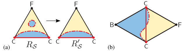
Fig. 12. Strong Consistency . (a) Simplification removes regions that do not intersect mesh edges. (b) For Strong Consistency, the true contour does not necessarily coincide with the CC edge, but cannot intersect the FC or BC edges. Figure 19 shows a case where it does.
