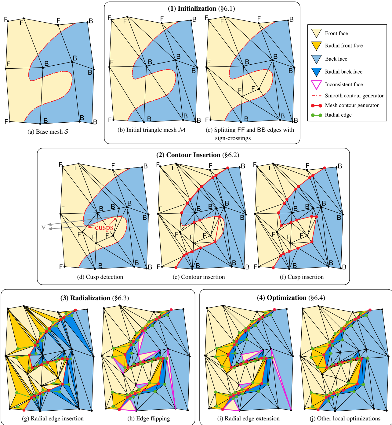
Fig. 15. Overview of the mesh generation algorithm. (a) Starting from the base mesh of \mathcal{S} , (b) the mesh \mathcal{M} is initialized by splitting all quads into triangles and (c) every FF and BB edges with sign-crossings. Contours are then inserted in the mesh by 3 subphases: (d) cusps detection, (e) contour edges insertion and (f) cusp insertion. The radialization step first (g) inserts radial edges in the mesh, before (h) flipping edges to convert every face touching the contour into a radial triangle. Consistency of the mesh is finally improved by (i) extending radial edges and (j) local perturbations.
