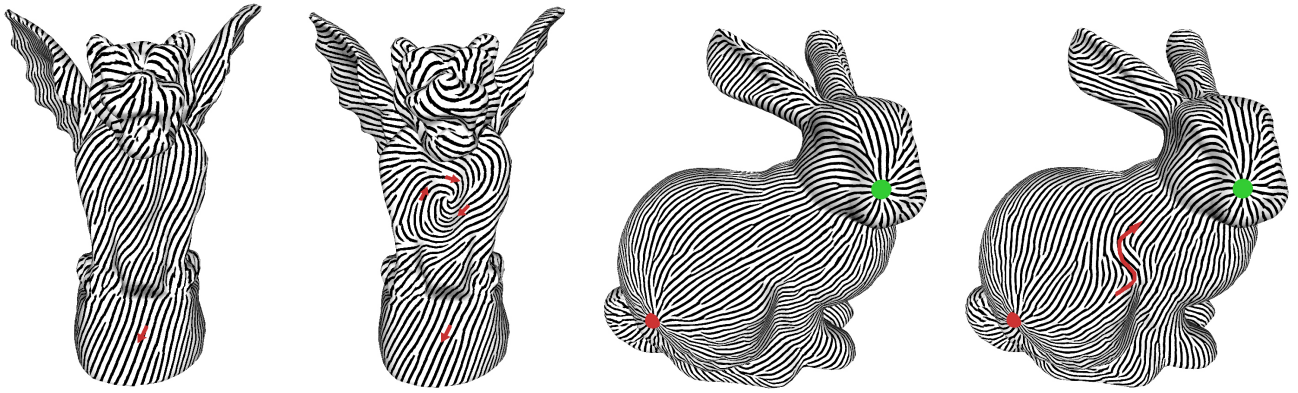
Figure 8: On the gargoyle model, a single edge constraint induces a global field; adding 3 closely spaced edge constraints creates a spiral. On the bunny model, a single source/sink pair produces the field on the left which is then reshaped with a curve constraint drawn on the body.
