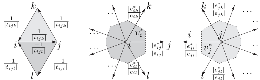
Figure 6: The 1-form Laplace stencil, Eq. (18), for a given e_{ij} depends on data at the two incident triangles (left) as well as the edges incident on v_i and v_j (middle and right).
